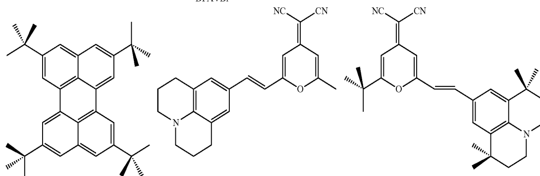
TBPe
