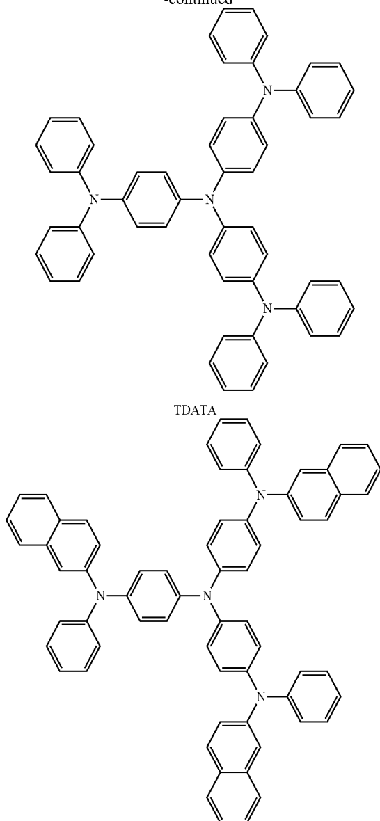
2-TNATA
