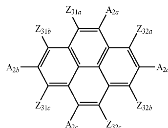
Formula 2A(1)
