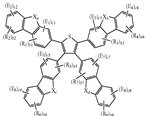
Formula 1-3(1)
