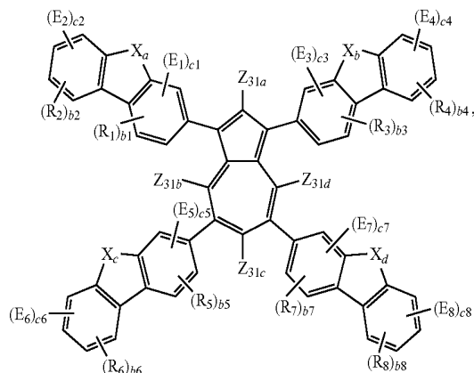
Formula 1-4(1)
