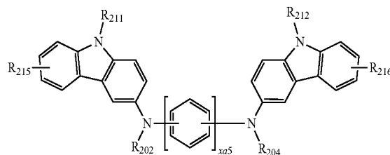
Formula 202A
