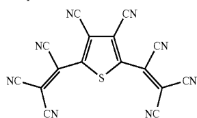
Compound C
