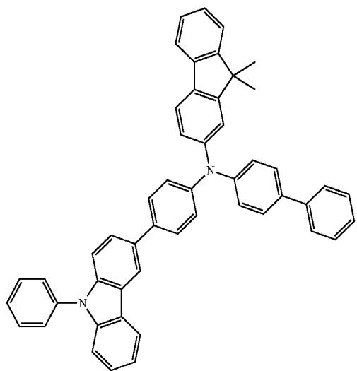
HT21
