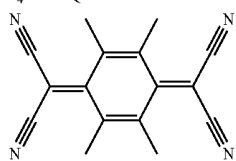
Compound A
