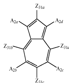
Formula 2A
