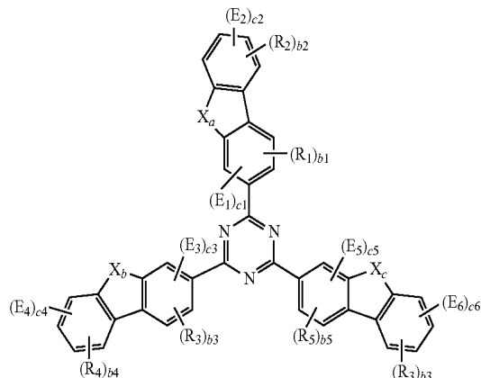
Formula 1-1(1)
