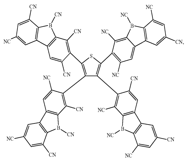
Compound 3
