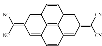
HT21
